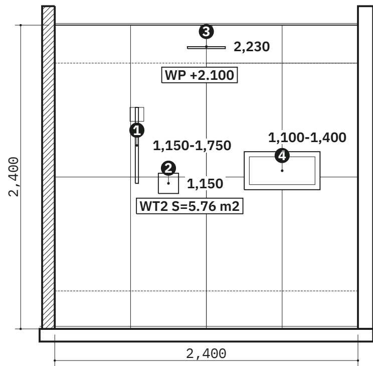
1 ELEVATION 1 - NORTH WALL 1:30
