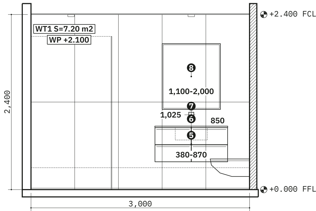
2 ELEVATION 2 - EAST WALL 1:30
