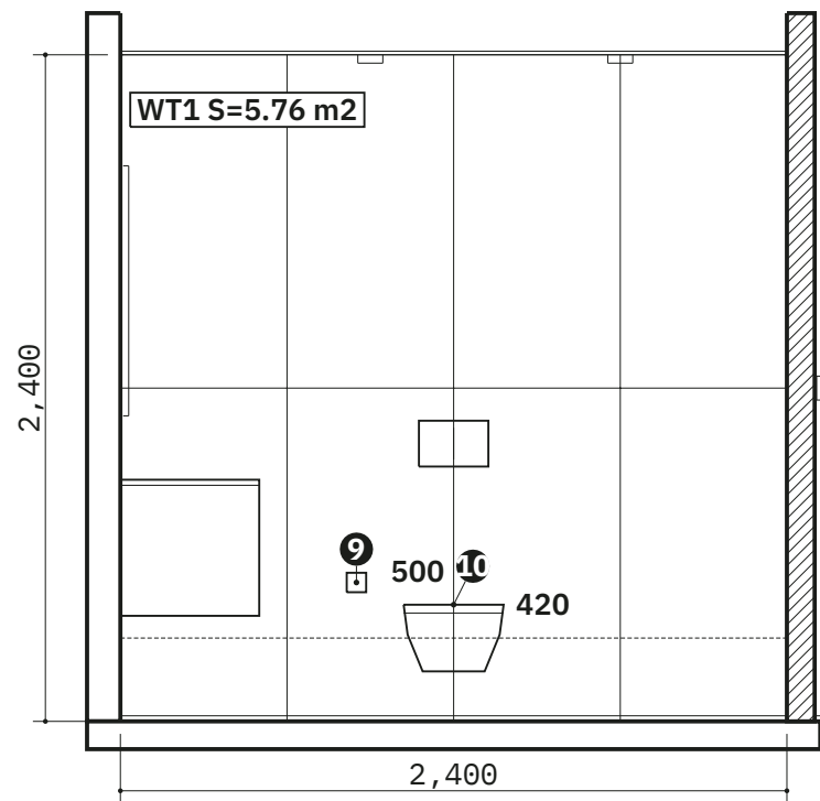
3 ELEVATION 3 - SOUTH WALL 1:30
