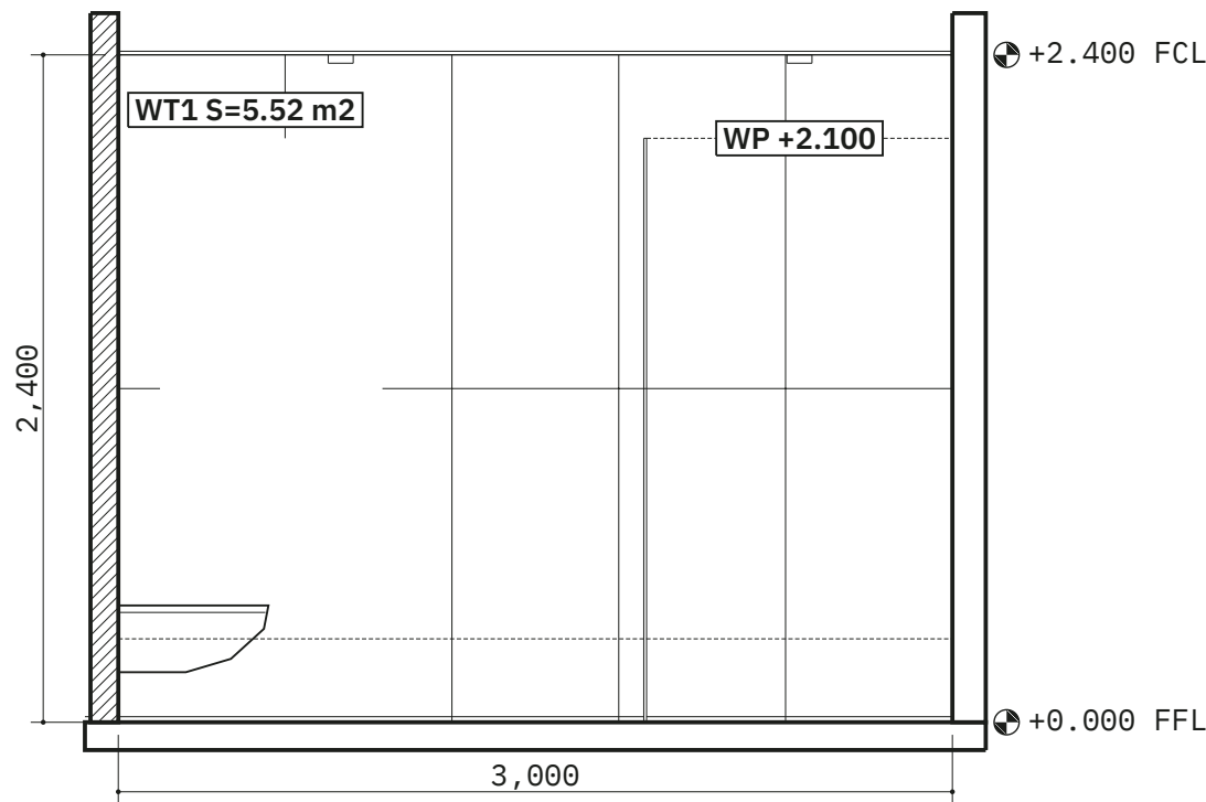
4 ELEVATION 4 - WEST WALL 1:30
